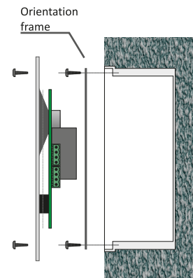
Embedded mounting in solid partition Box: Ref. UDE CW-93 (Not included)
